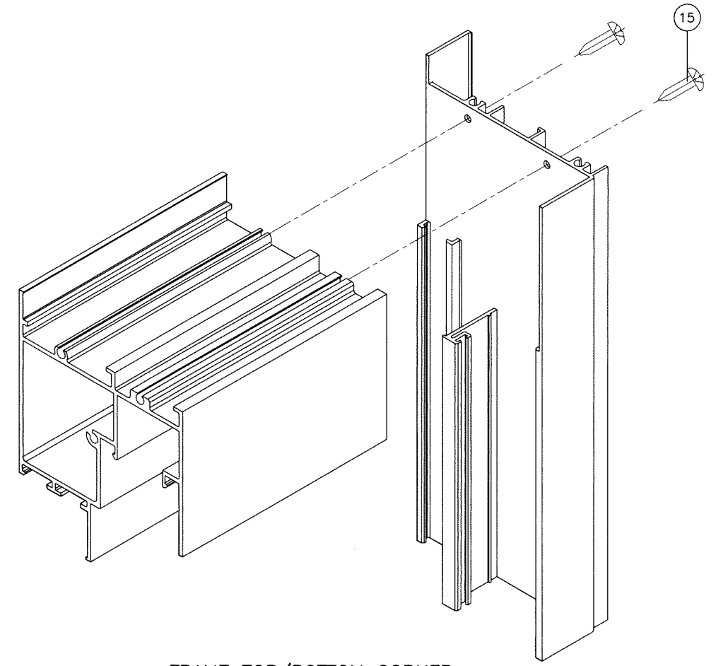
FRAME TOP/BOTTOM CORNER
